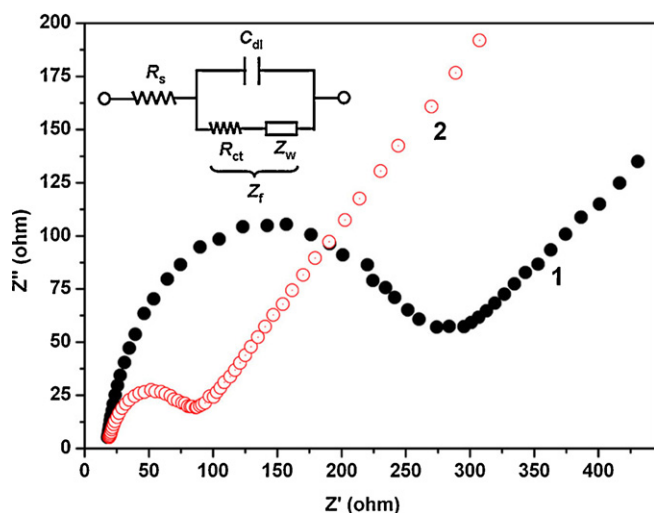
Fig. 6. Electrochemical impedance spectroscopy (EIS) of 10 mM \text{Fe}(\text{CN})_6^{3-/4-} in 1.0 M KCl using OMC-1 (curve 1) and OMC-2 (curve 2). The inset is the Randle equivalent circuit.
