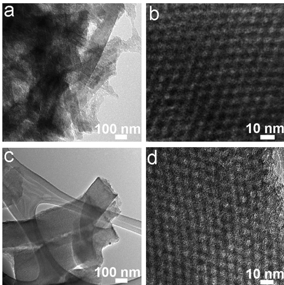
Fig. 2. TEM images of OMC-1 (a and b) and OMC-2 (c and d).
