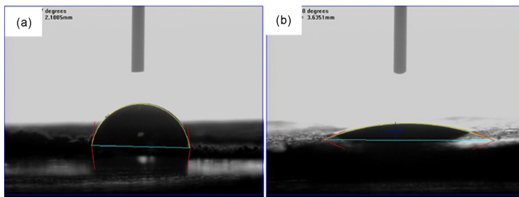
Fig. 4. Photographs of water droplet on OMC-1 (a) and OMC-2 (b).
