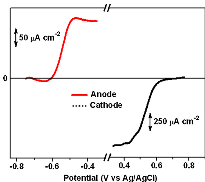
Fig. 8. Polarization curves of the anode (GOD/OMC-2 modified GCE electrode) in 10 mM glucose solution (in 100 mM PBS, pH 7.0) and the cathode (Pt wire) in 100 mM PBS with pH 1.0. The scan rate is 1 \text{ mV s}^{-1} .
