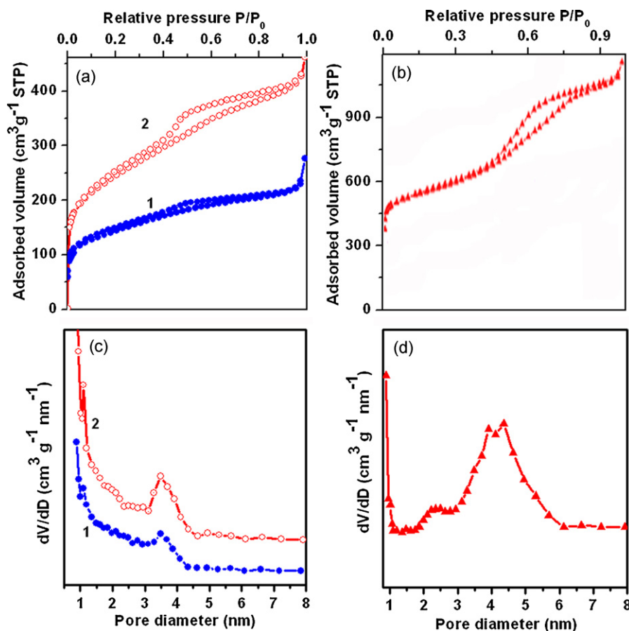
Fig. 3. Nitrogen adsorption/desorption isotherms of OMCs via microwave treated (a) and conventional method (b). The corresponding pore size distributions obtained from the desorption branch using the BJH method of OMCs microwave treated (c) and conventional method (d). Curve 1: OMC-1 and curve 2: OMC-2.
