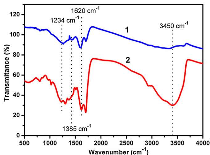
Fig. 5. FTIR spectra of OMC-1 (curve 1) and OMC-2 (curve 2).
