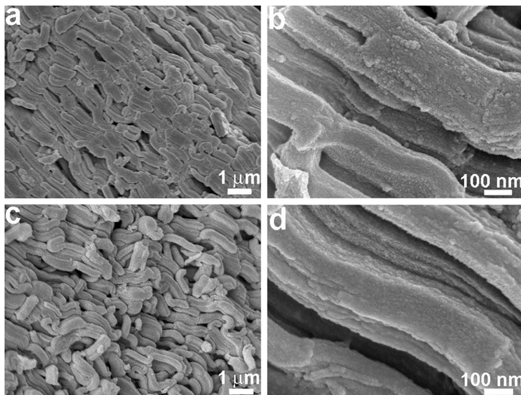
Fig. 1. FESEM images of OMC-1 (a and b) and OMC-2 (c and d).
