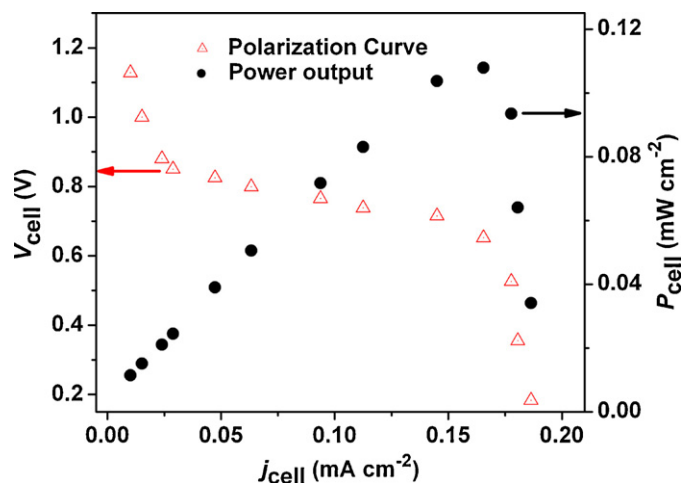
Fig. 9. Polarization curve of the assembled glucose/ \text{O}_2 biofuel cell and the dependence of the power output on the current density.
