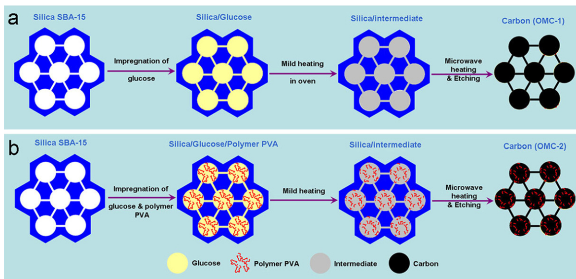
Scheme 1. Schematic representation of the preparation process of OMC-1 (a) and OMC-2 (b).
